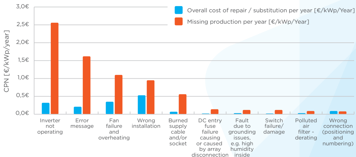
Figure 5: CPN, repair costs ( CPN_{\text{failure\_fix}} ) and performance losses ( CPN_{\text{never\_detected}} ) for top 10 risks for PV inverters of all system sizes
