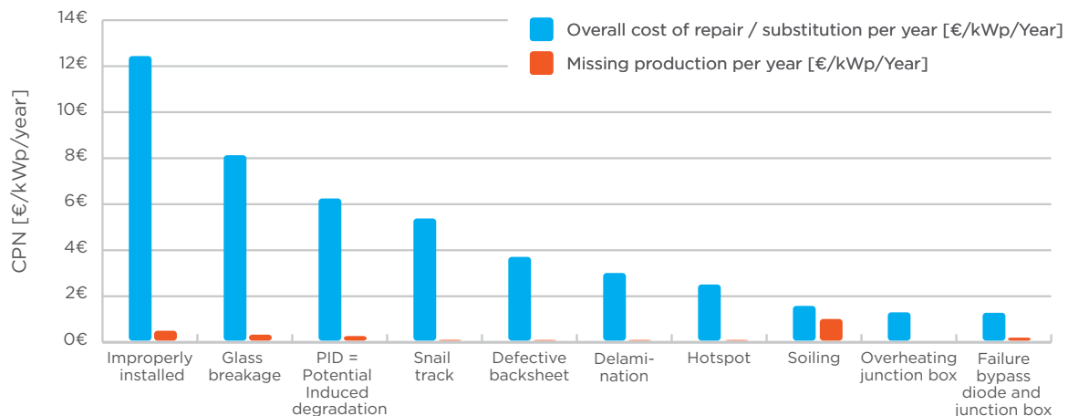
Figure 4: CPN, repair costs ( CPN_{\text{failure\_fix}} ) and performance losses ( CPN_{\text{never\_detected}} ) for top 10 risks for PV modules of all system sizes
